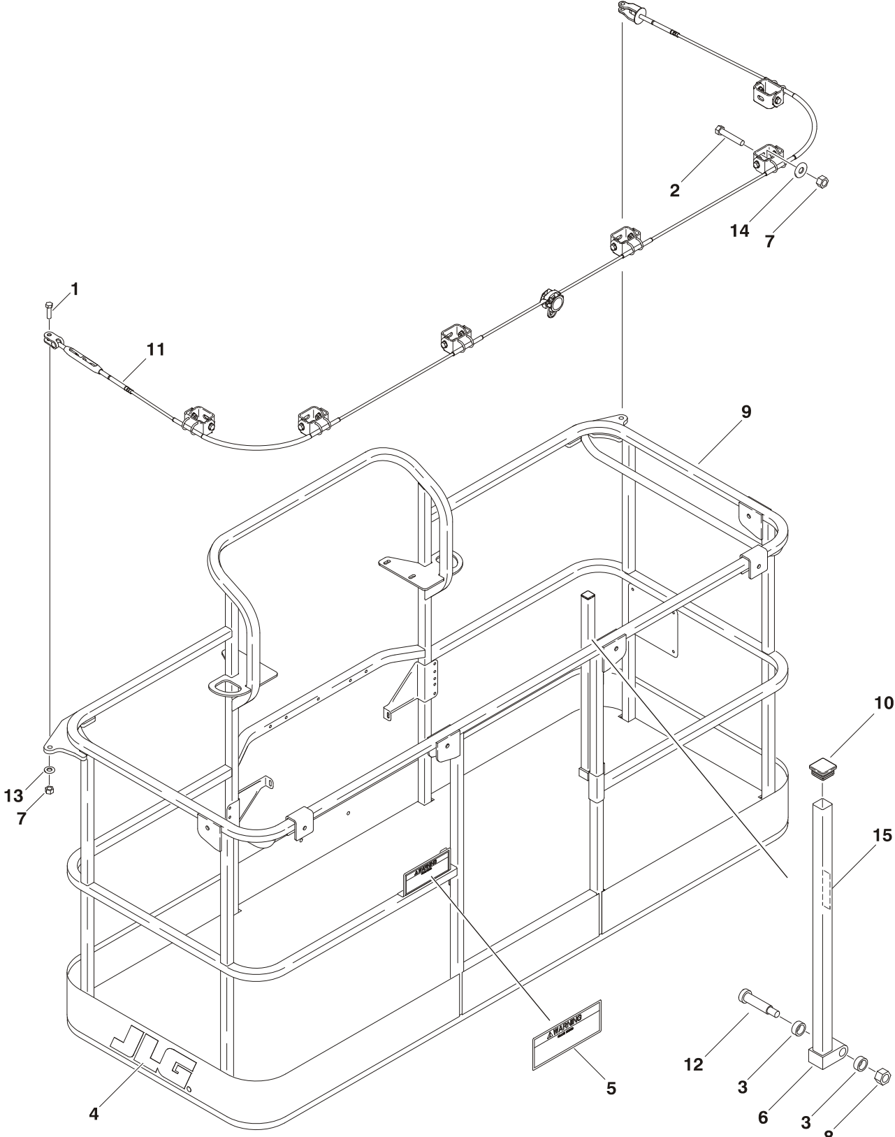
FIGURE 4-2. PLATFORM COMPONENTS INSTALLATION (FALL ARREST FOR PLATFORM)
