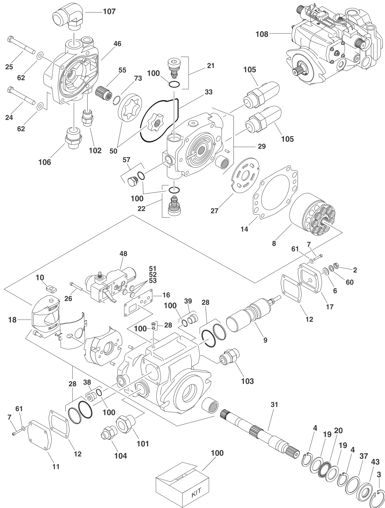
FIGURE 2-11. PISTON PUMP ASSEMBLY (EATON)
