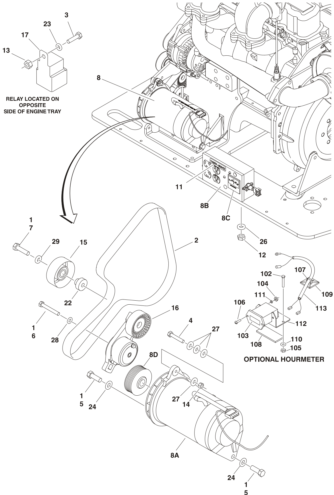
FIGURE 2-22. 2500W GENERATOR INSTALLATION - GM MACHINES (OPTIONAL)
