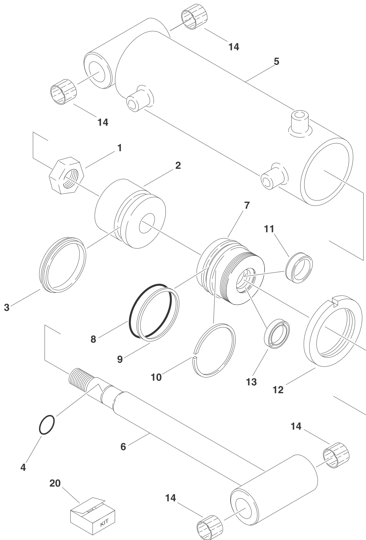
FIGURE 5-10. STEER CYLINDER ASSEMBLY (USA BUILT MACHINES SN 0300140000 TO SN 0300142666)
