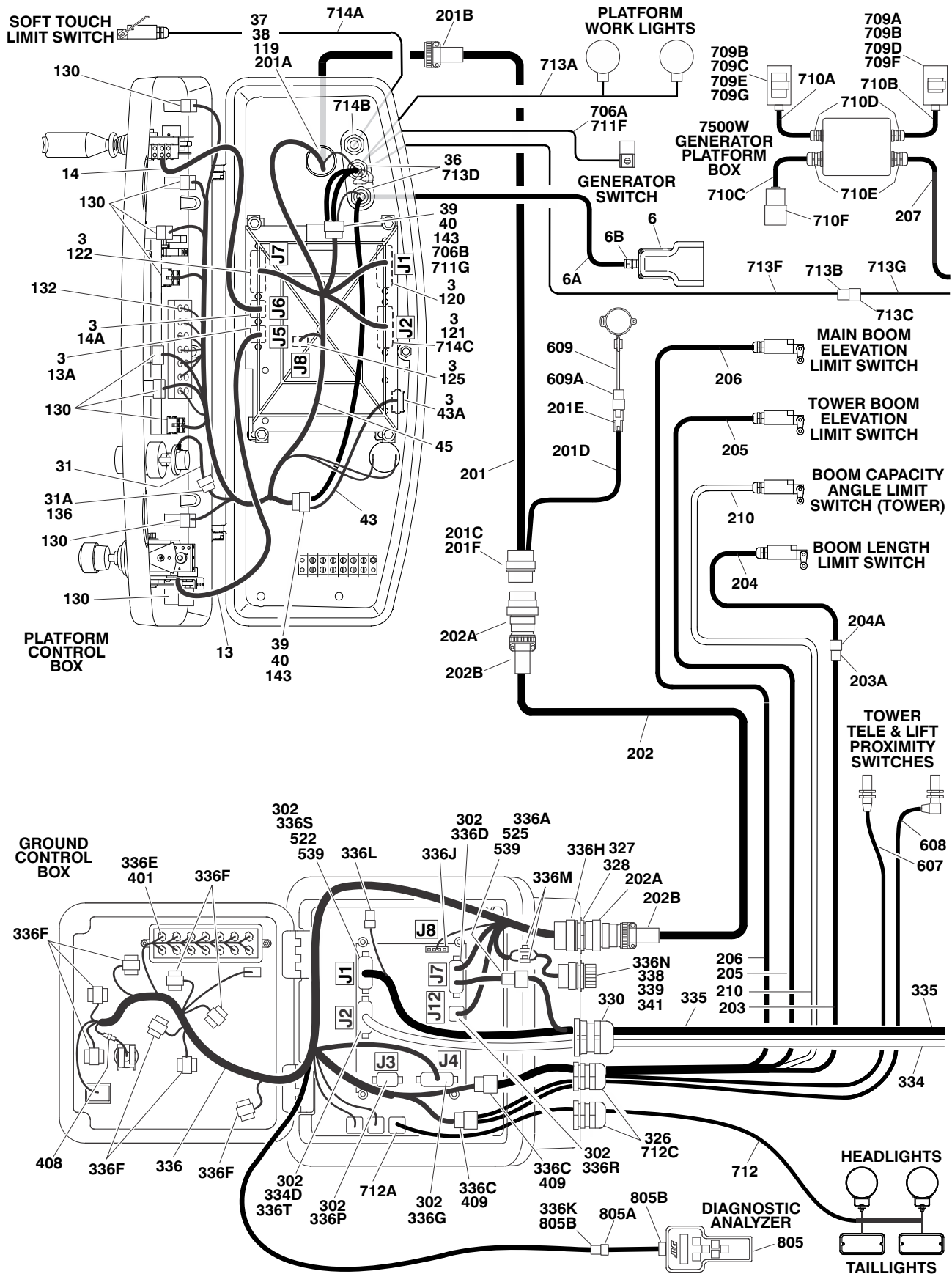
FIGURE 7-2. HARNESS COMPONENTS INSTALLATION
