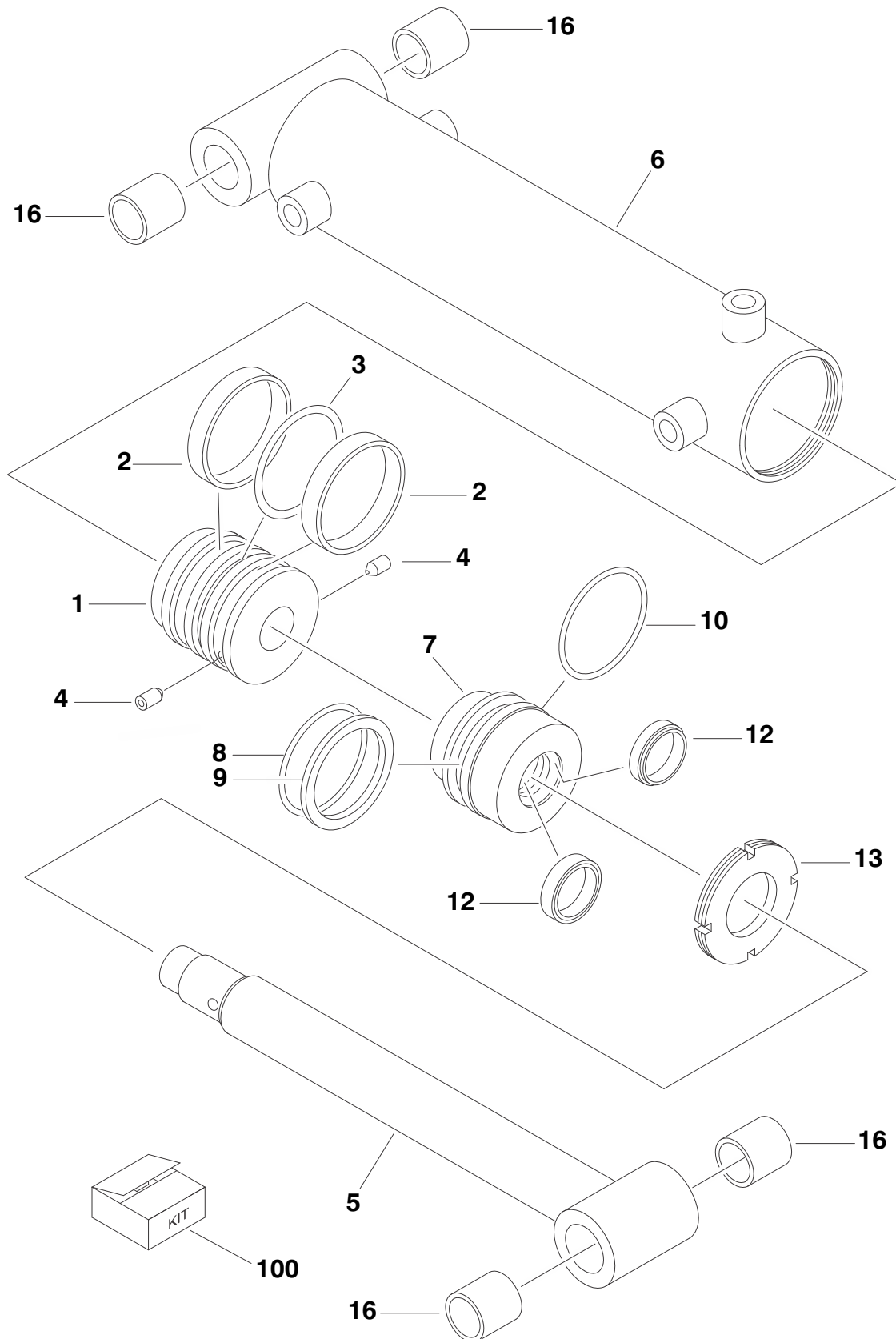
FIGURE 5-11. STEER CYLINDER ASSEMBLY (USA BUILT MACHINES SN 0300142664 TO SN 030183033 ONLY & CHINA BUILT MACHINES SN B300000100 TO PRESENT ONLY)
