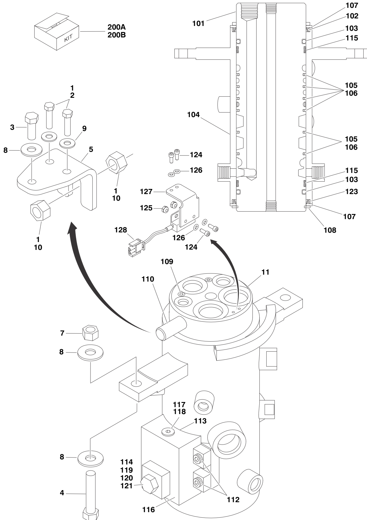
FIGURE 2-14. ROTARY COUPLING INSTALLATION
