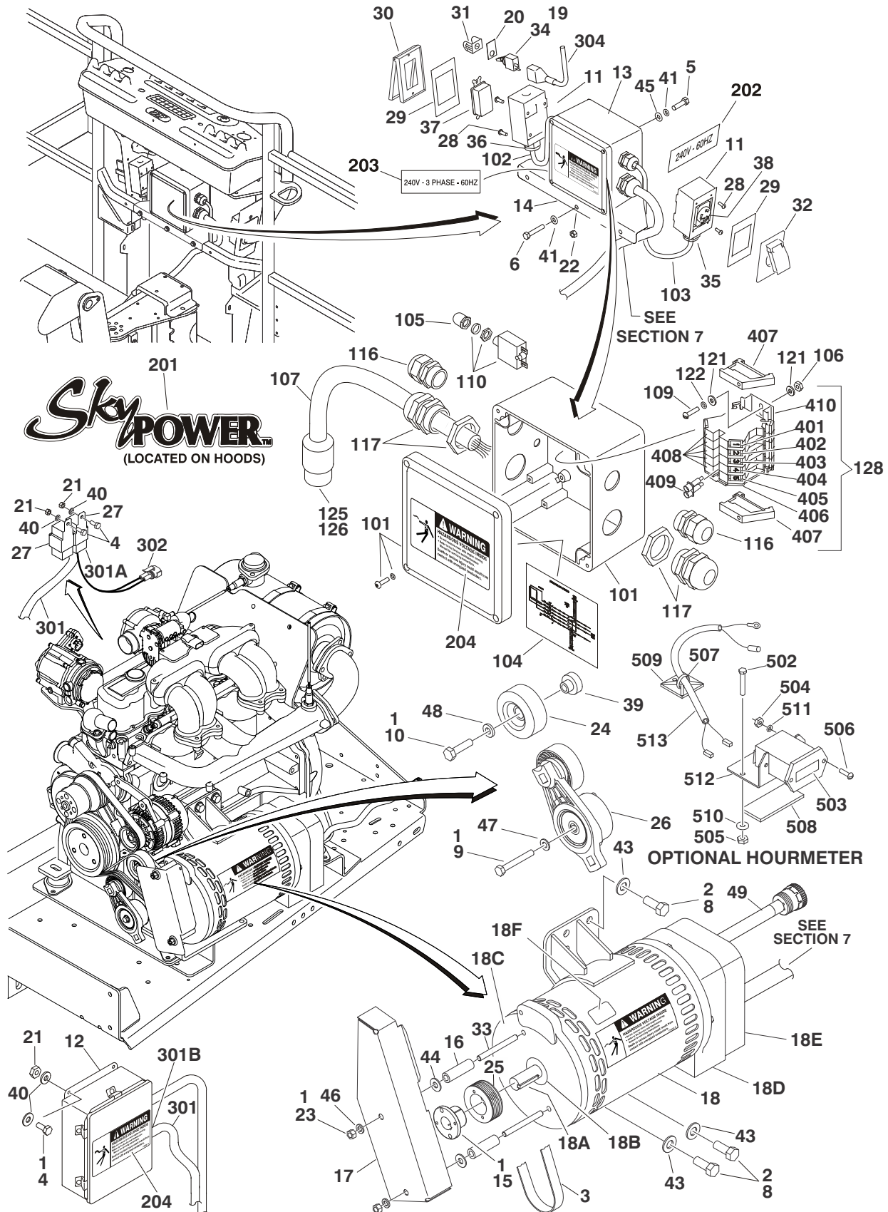
FIGURE 2-24. 7500W SKYPOWER GENERATOR INSTALLATION - GM MACHINES
