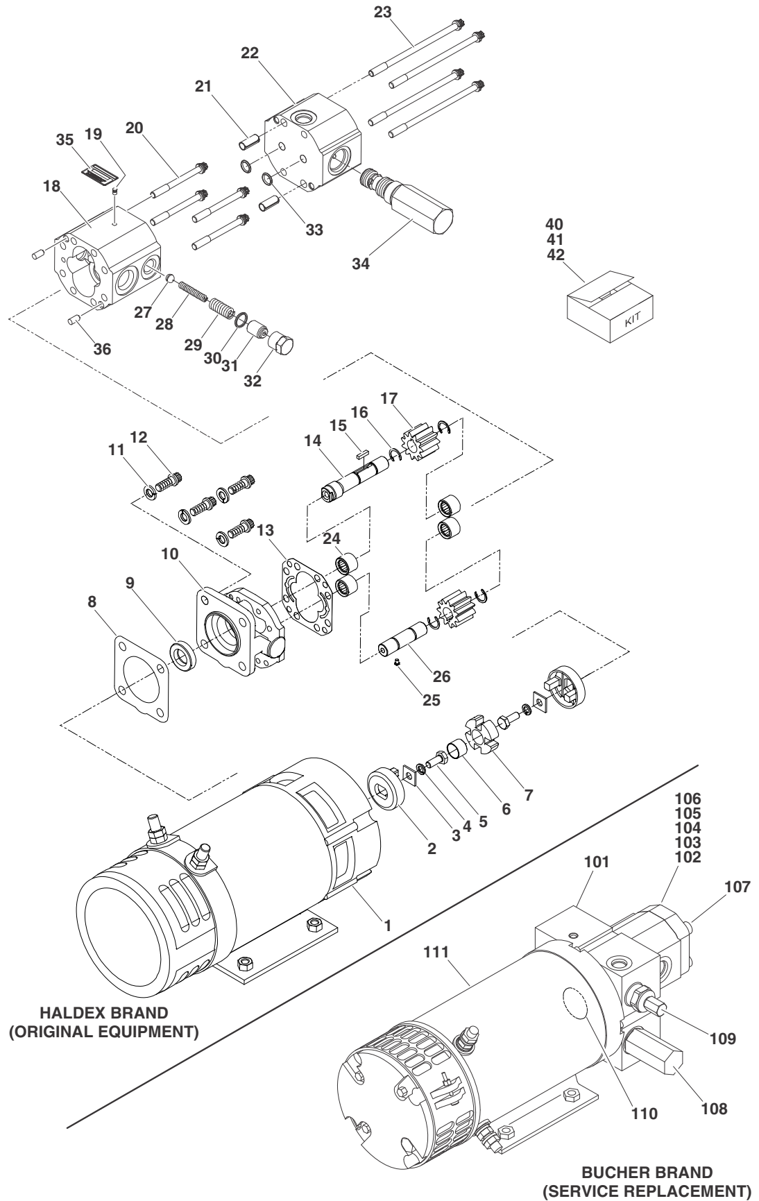
FIGURE 2-4. AUXILIARY PUMP ASSEMBLY
