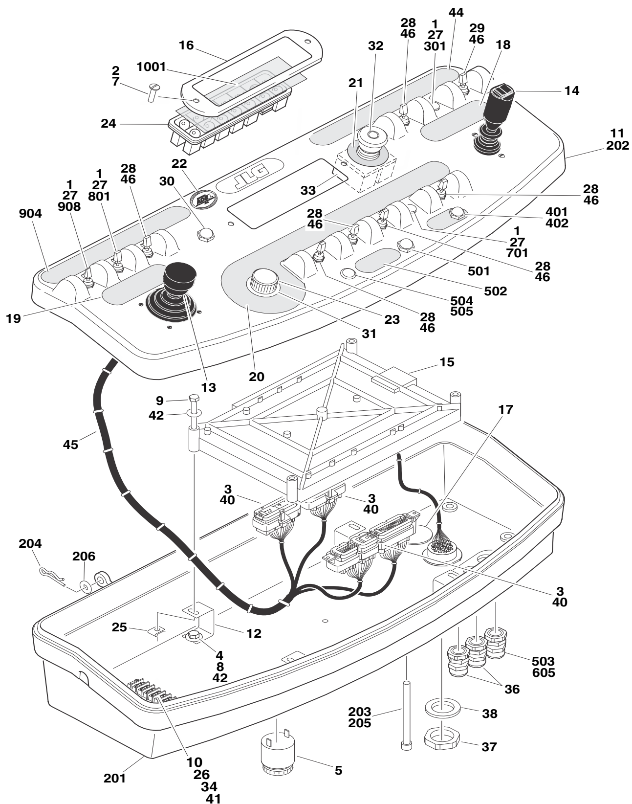
FIGURE 4-3. PLATFORM CONSOLE ASSEMBLY
