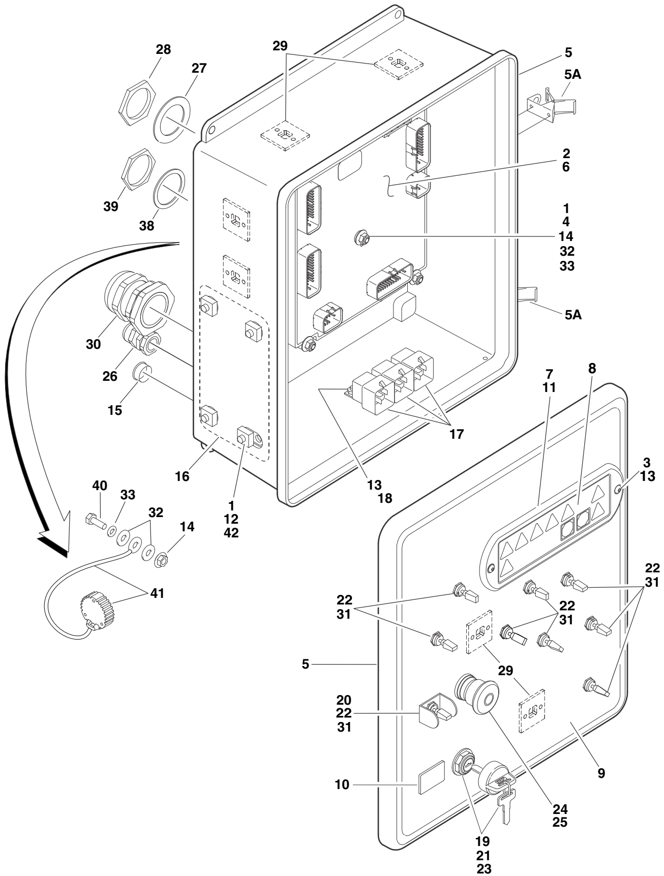
FIGURE 2-15. GROUND CONTROL BOX ASSEMBLY
