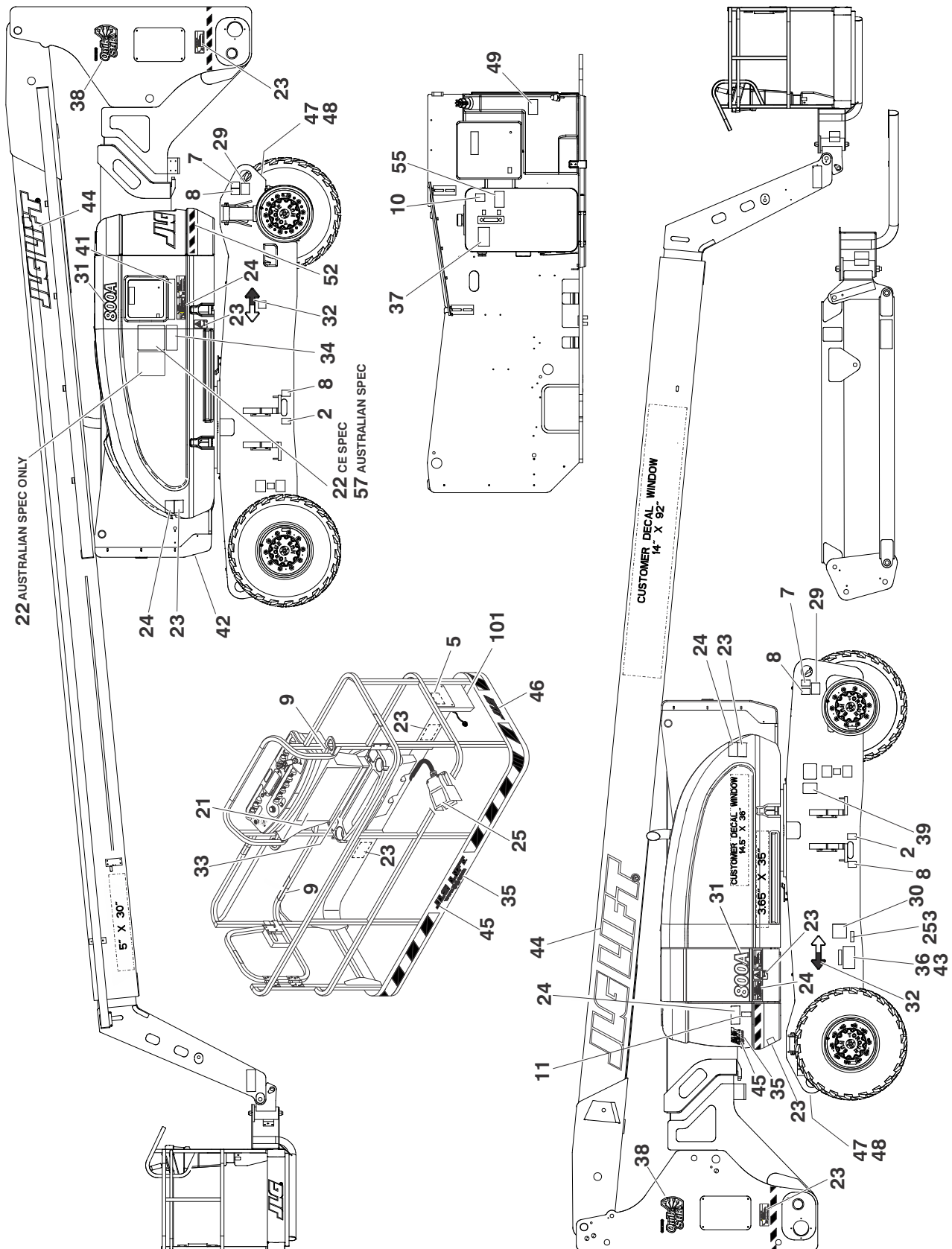
FIGURE 8-3. DECAL INSTALLATION (AUSTRALIAN & CE SPEC)
