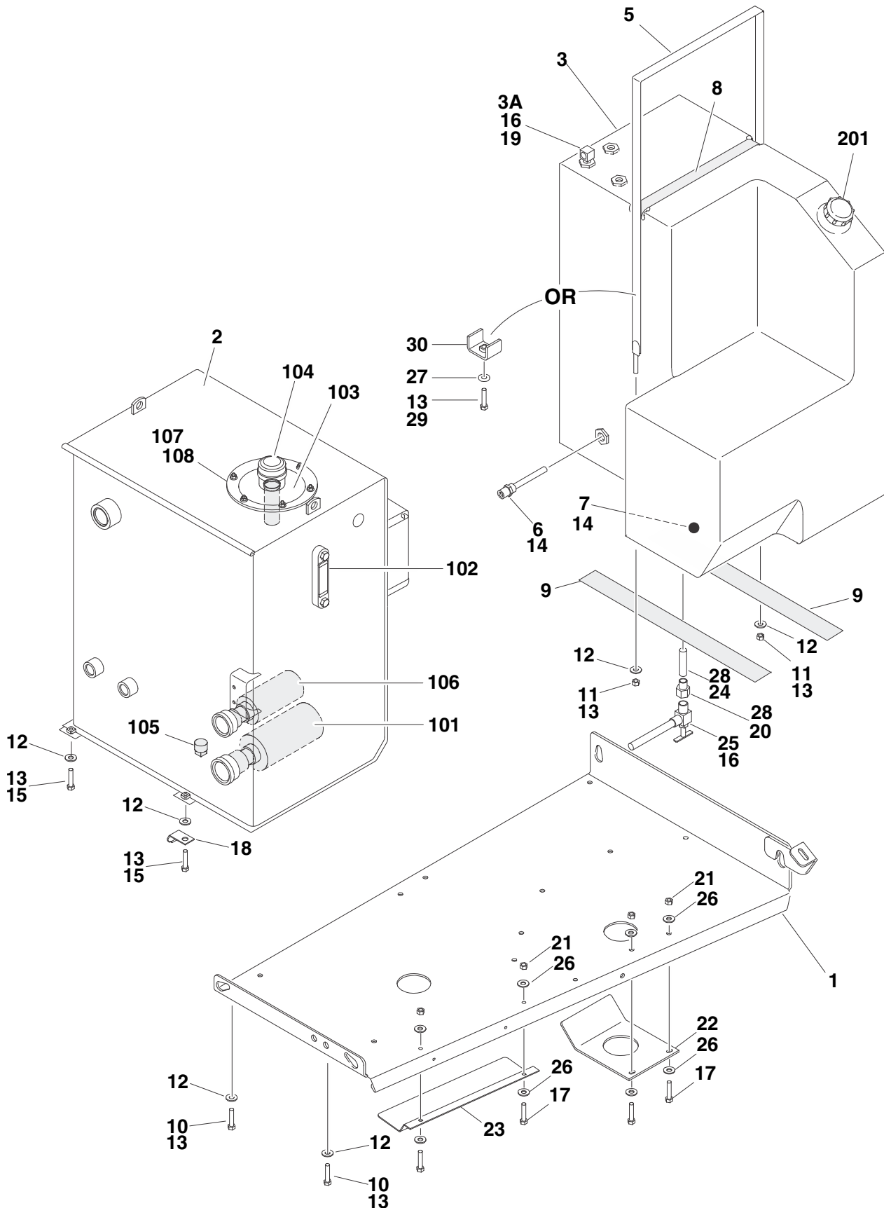
FIGURE 2-12. TANK INSTALLATIONS
