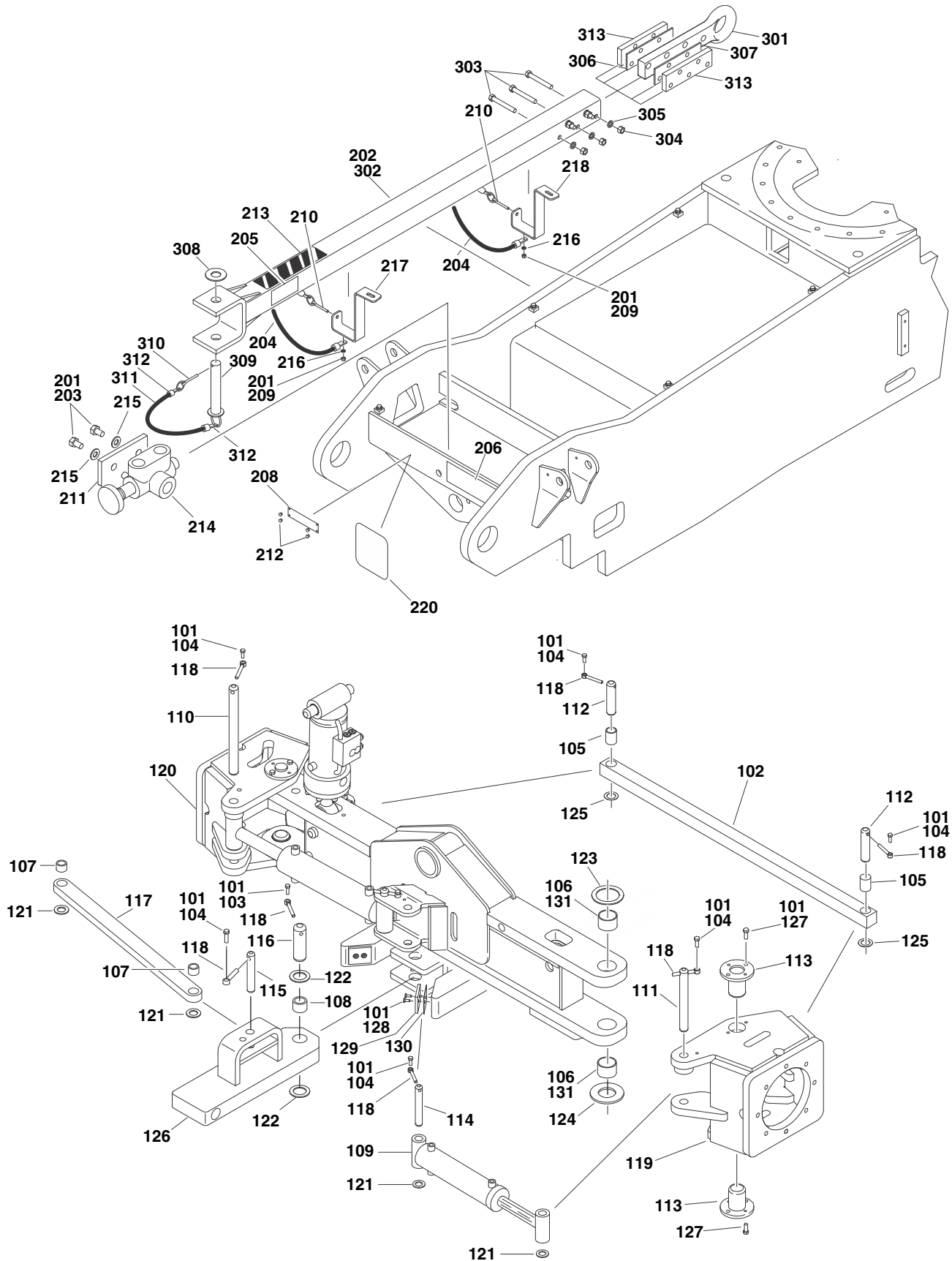
FIGURE 1-6. TOW PACKAGE INSTALLATION (2WS ONLY) (ANSI, ANSI EXPORT & CE)
