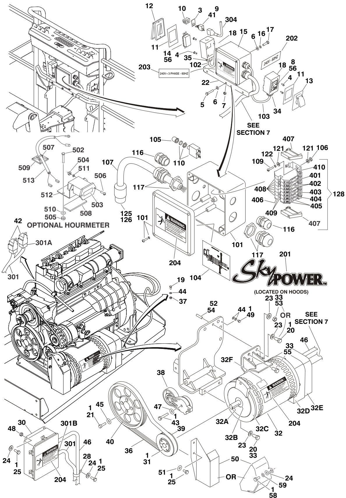
FIGURE 2-23. 7500W SKYPOWER GENERATOR INSTALLATION - CATERPILLAR AND DEUTZ MACHINES
