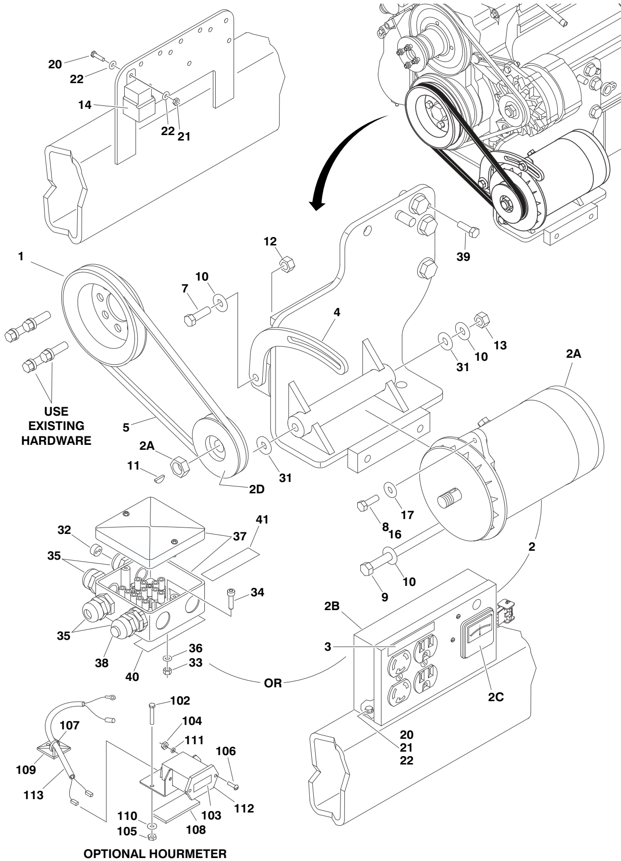
FIGURE 2-21. 2500W GENERATOR INSTALLATION - DEUTZ MACHINES (OPTIONAL)
